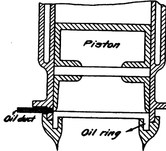
FIG. 44.—Oil Ring.
